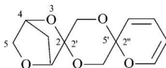
3,6-dioksadispiro[bicyklo[2.2.1]heptano-2,2'-[1,4]dioksano-5',2''-piran] (PIN)
