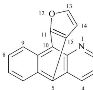
10,5-[2,3]furanobenzo[g]chinolina (PIN)
