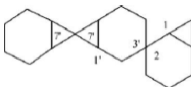
2,3':7',7''-dispiroter[bicyclo[4.1.0]heptan] (PIN)
