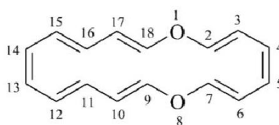
1,8-dioksacyklooktadekyn 1,8-dioksacyklooktadeka-2,4,6,9,11,13,15,17-oktaen (PIN)
