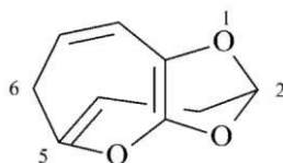
2H,6H-2,5-(epietanyloylideno)[1,3]dioksolo[4,5-b]oksepin (PIN)
