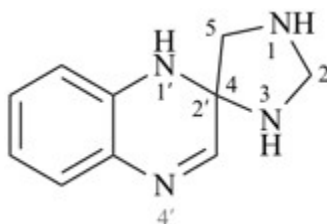
1'H-spiro[imidazolidyno-4,2'-chinoksalina] (PIN)
