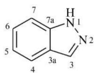
(17) indazol (pokazano izomer 1 H ; PINem jest: 1 H -indazol)
