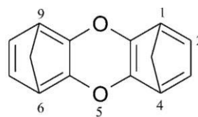
1,4:6,9-dimetanooksoantren (PIN) 1,4:6,9-dimetanodibenzo[ b,e ]dioksyn
