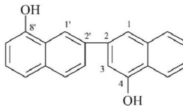
[2,2'-binaftaleno]-4,8'-diol (PIN) 3,7'-bi-1-naftol
