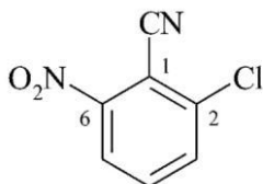
2-chloro-6-nitrobenzonitryl (PIN)
