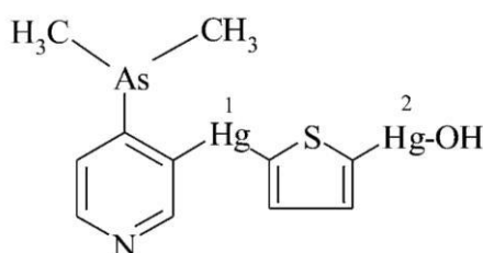
1-[4-(dimetyloarsanylo)pyrydyn-3-ylo]-2-hydroksydo-μ-tiofeno-2,5-diylodirtęć
