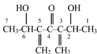
2,6-dihydroksy-3,5-dimetylidenoheptan-4-on (PIN)
