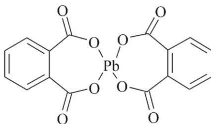
3,3'-spirobi[[2,4,3]benzodioxapbino]-1,1',5,5'-tetraon (PIN)
