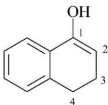
(1) 3,4-dihydronaftalen-1-ol (PIN)
