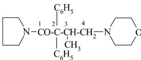
3-metylo-4-(morfolin-4-ylo)-2,2-difenylo-1-(pirolidyn-1-ylo)butan-2-on (PIN)
