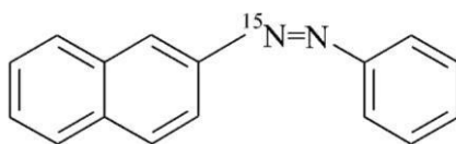
1-(naftalen-2-ylo)-2-fenylo(1- ^{15}\text{N} )diazen (PIN) naftaleno-2-( ^{15}\text{N}=\text{N} )azobenzen
