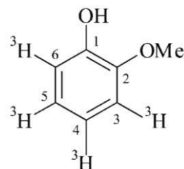
2-metoksy(3,4,5,6- 3 H 4 )fenol (PIN)
