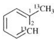
1-( 13 C)metylo(2- 13 C)benzen (PIN) ( \alpha,2 - 13 C 2 )-toluen
