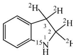
2,3-di[( 2 H)hydro](2,3- 2 H 2 , 15 N)-1 H -indol (PIN) [nie (2,3- 2 H 2 )dihydro(2,3- 2 H 2 , 1- 15 N)-1 H -indol]
