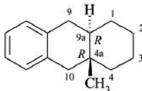
(4a R ,9a R )-4a-metylo-1,2,3,4,4a,9,9a,10-oktahydroantracen (PIN)
