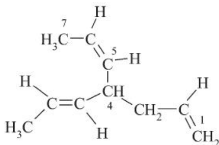
(5 Z )-4-[(1 E )-prop-1-en-1-yl]hepta-1,5-dien (PIN)
