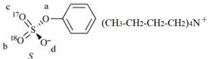
(S)-[ O -fenylo( 17 O 1 , 18 O 1 )siarczan] N,N,N -tributylobutano-1-aminium (PIN)
