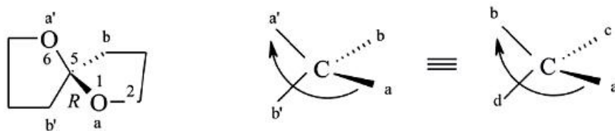
(5R)-1,6-dioksaspiro[4.4]nonan (PIN)
