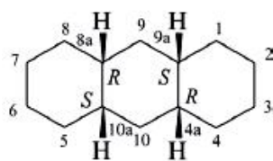
(4a R ,8a R ,9a S ,10a S )-tetradekahydroantracen (PIN)
