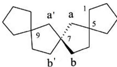
(7S)-trispino[4.1.1.4 9 .2 7 .2 5 ]heptadekan (PIN)
