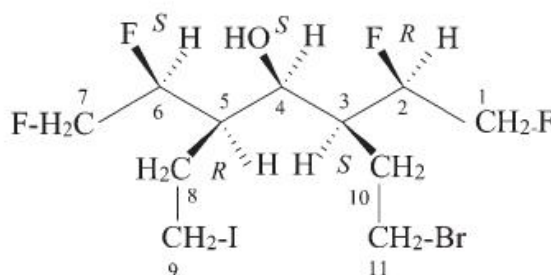
(2R,3S,4S,5R,6S)-3-(2-bromoetylo)-1,2,6,7-tetrafluoro-5-(2-jodoetylo)heptan-4-ol (PIN)
