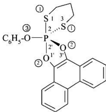
(TBPY-5-12-C)-2-fenoksy-2H-2 \lambda^5 -spiro[[1,3,2]-ditiafosfinano-2,2'-fenantro[9,10-d][1,3,2] dioksafosfol] (PIN)
