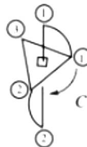
(TBPY-5-12-C)-2-fenoksy-2H-2 \lambda^5 -spiro[[1,3,2]-ditiafosfinano-2,2'-fenantro[9,10-d][1,3,2] dioksafosfol] (PIN)
