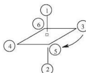
OC-6-24-C
