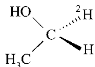
(1 R )-(1- 2 H 1 )etanol (PIN)
