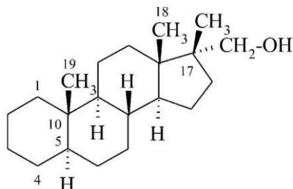
(17 \beta -metylo-5 \alpha -androstan-17 \alpha -ylo)metanol [nie (21-nor-5 \alpha -pregnan-17 \alpha -ylo)metanol]
