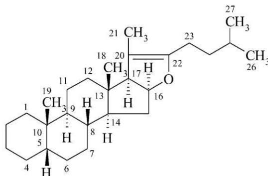
5β-furost-20(22)-en
