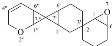
2'',7'-dioksa-2,3':7',7''-dispiroter[bicyclo[4.1.0]heptan]-4''-en (PIN)
