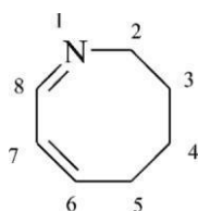
2,3,4,5-tetrahydroazocin (PIN)
