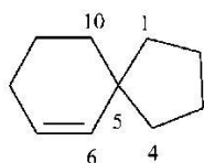
spiro[4.5]dek-6-en (PIN)
