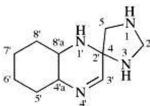
4',5',6',7',8',8'a-heksahydro-1'H-spiro[imidazolino-4,2'-chinoksalina] (PIN)
